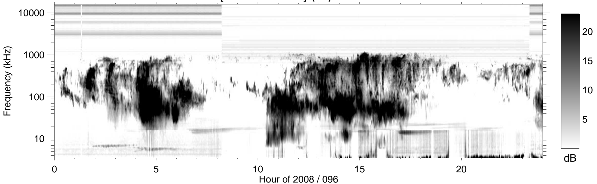
RPWS [ABCH1H2/Ex] (-B) 2008/04/05
