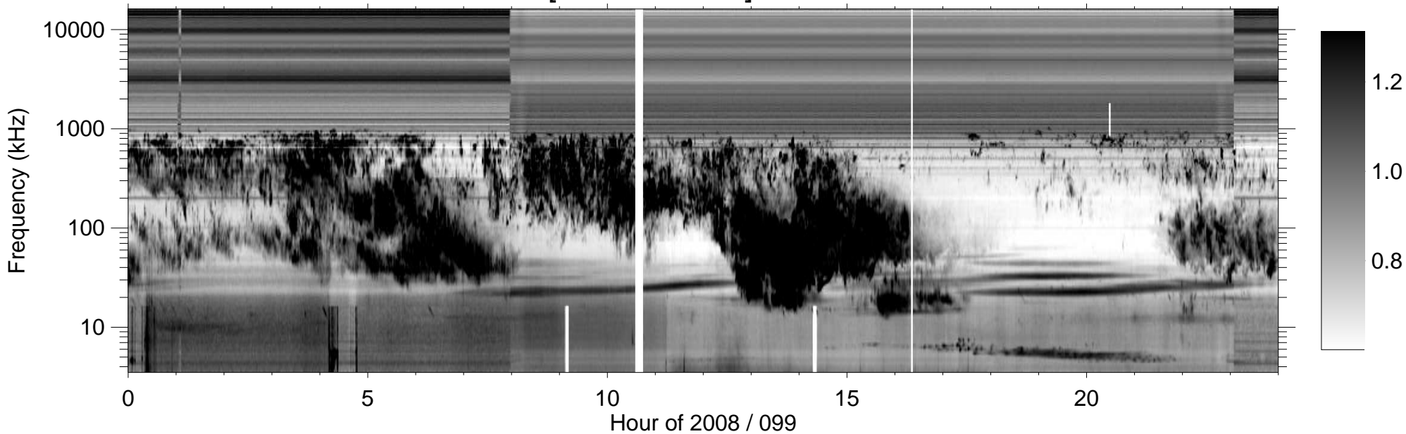
RPWS [ABCH1H2/Ex] (-B) 2008/04/08
