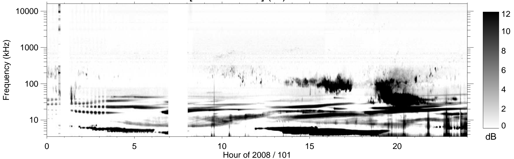
RPWS [ABCH1H2/Ex] (-B) 2008/04/10
