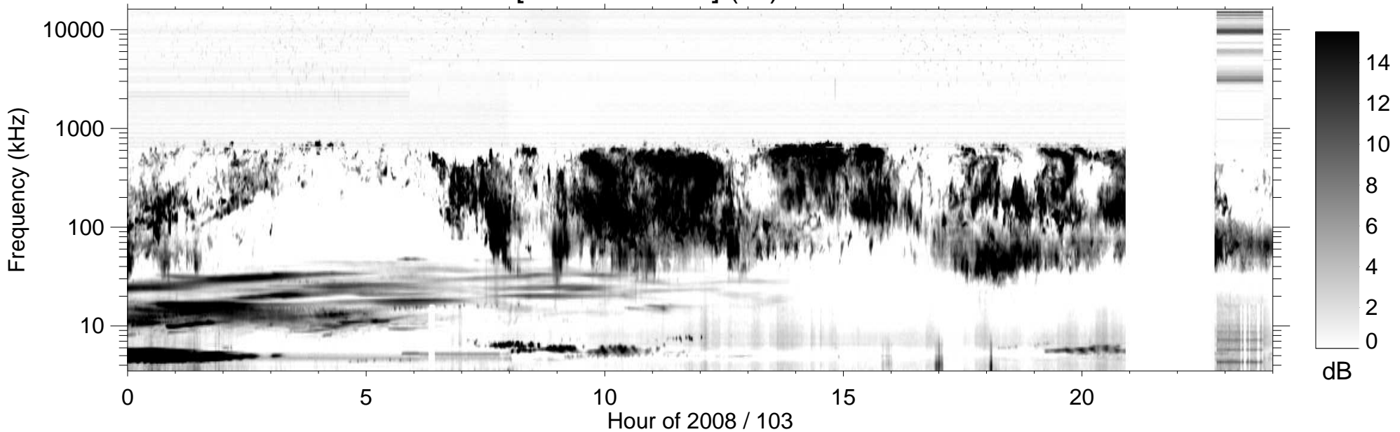
RPWS [ABCH1H2/Ex] (-B) 2008/04/12
