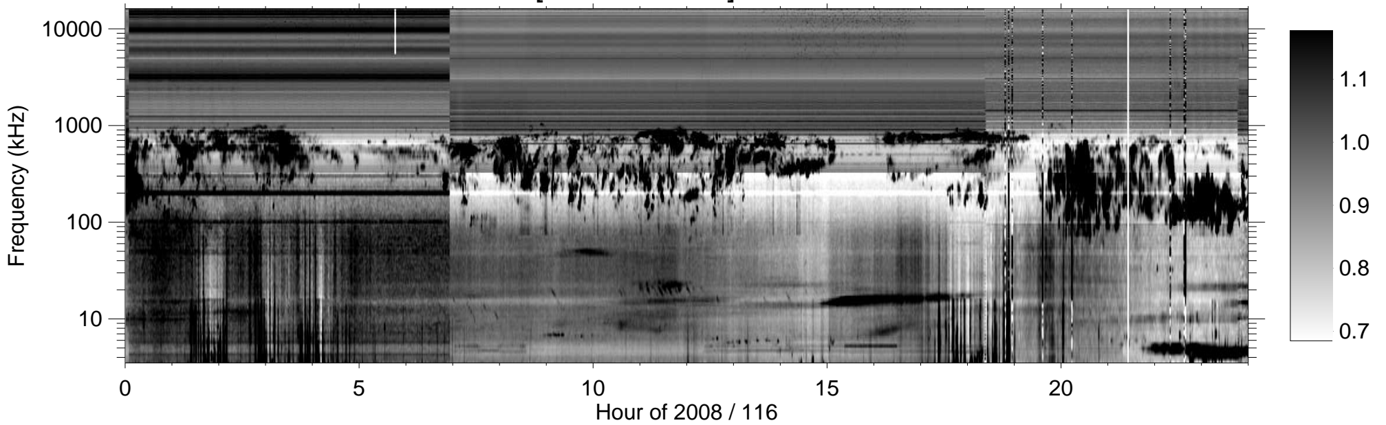
RPWS [ABCH1H2/Ex] (-B) 2008/04/25
