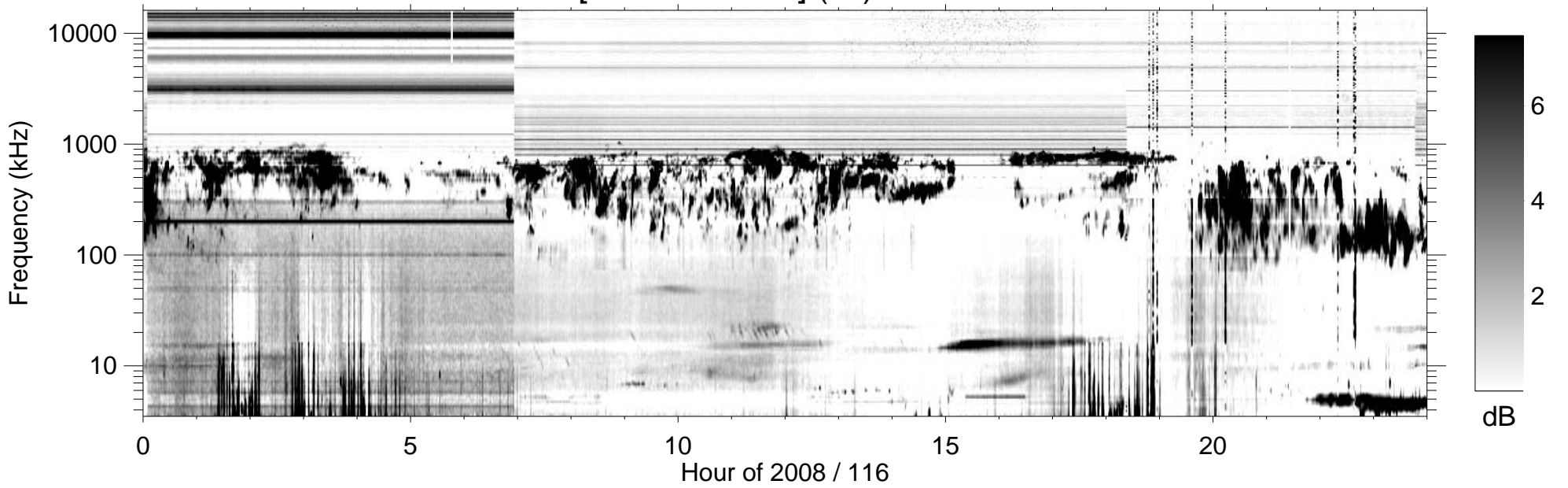
RPWS [ABCH1H2/Ex] (-B) 2008/04/25
