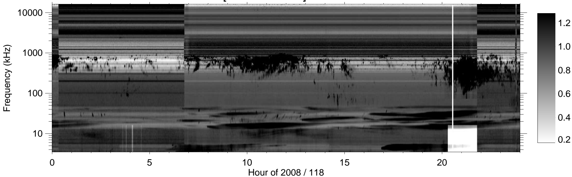
RPWS [ABCH1H2/Ex] (-B) 2008/04/27
