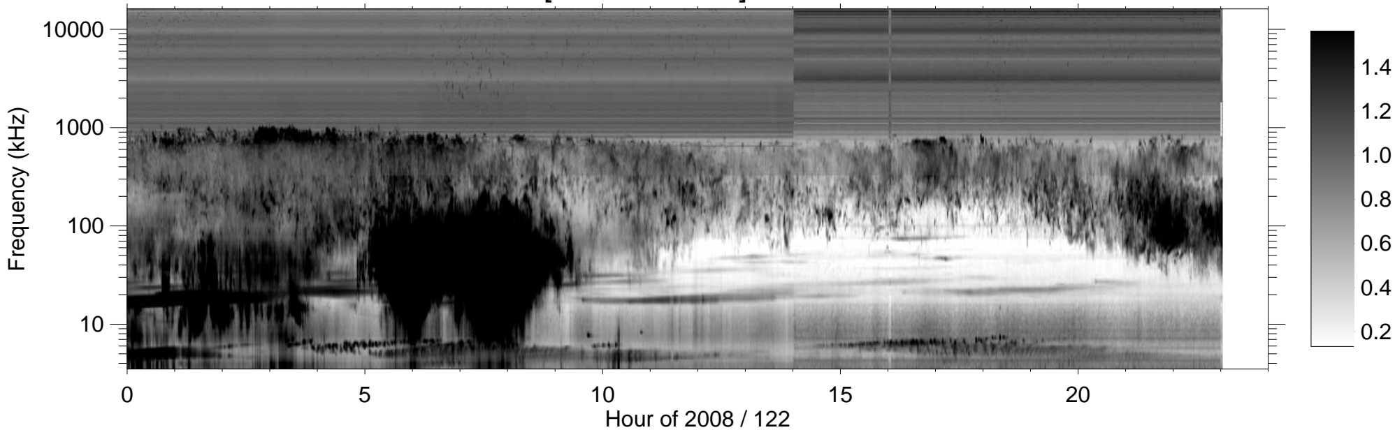
RPWS [ABCH1H2/Ex] (-B) 2008/05/01
