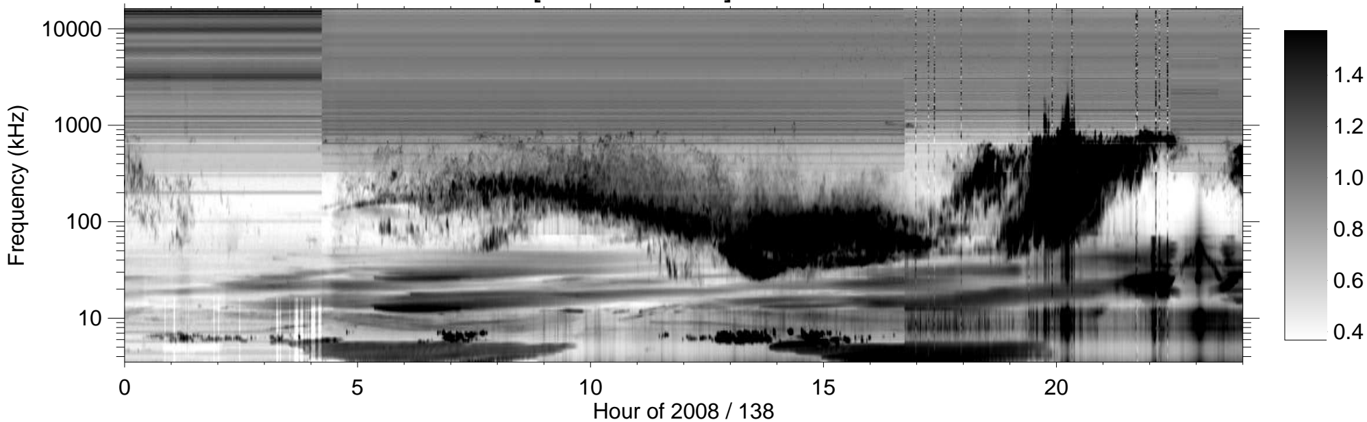
RPWS [ABCH1H2/Ex] (-B) 2008/05/17
