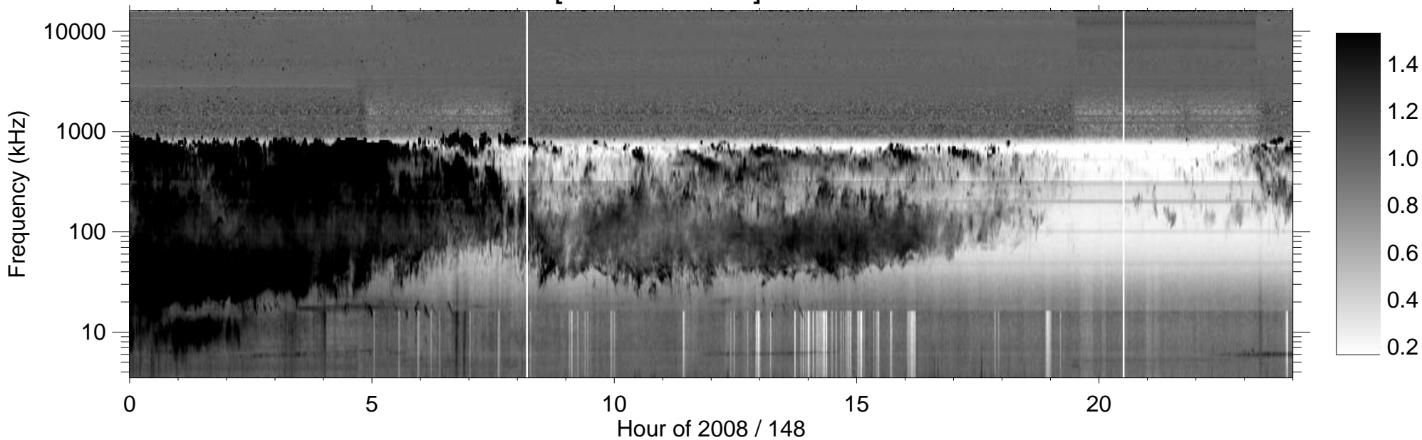
RPWS [ABCH1H2/Ex] (-B) 2008/05/27
