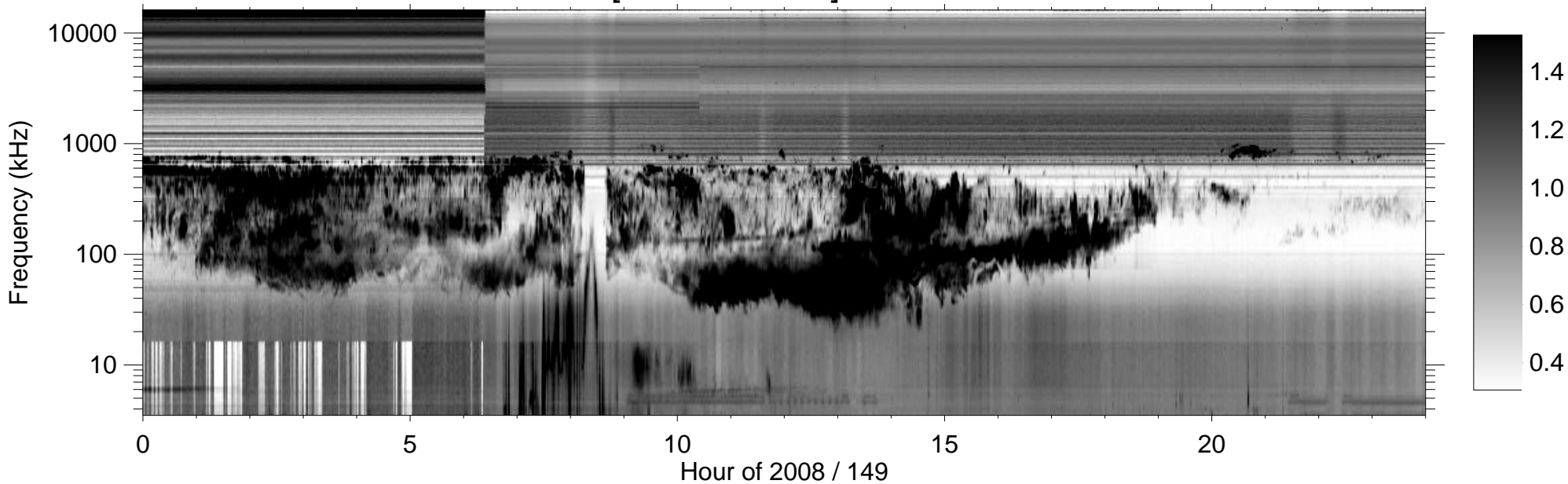
RPWS [ABCH1H2/Ex] (-B) 2008/05/28
