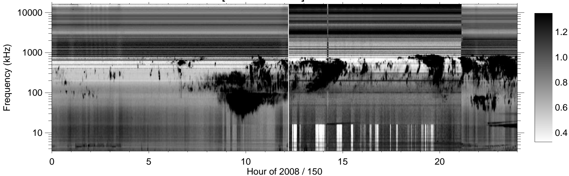
RPWS [ABCH1H2/Ex] (-B) 2008/05/29
