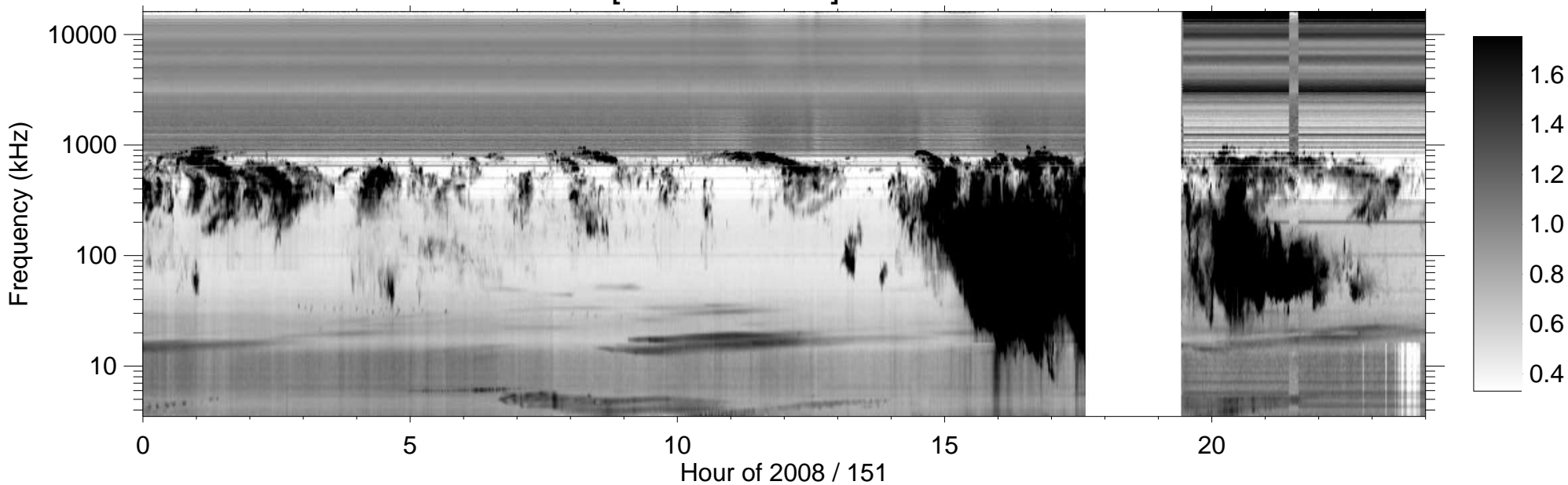
RPWS [ABCH1H2/Ex] (-B) 2008/05/30
