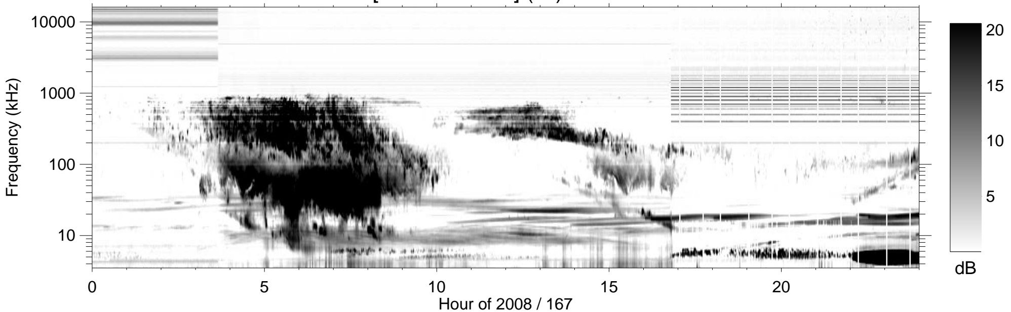
RPWS [ABCH1H2/Ex] (-B) 2008/06/15
