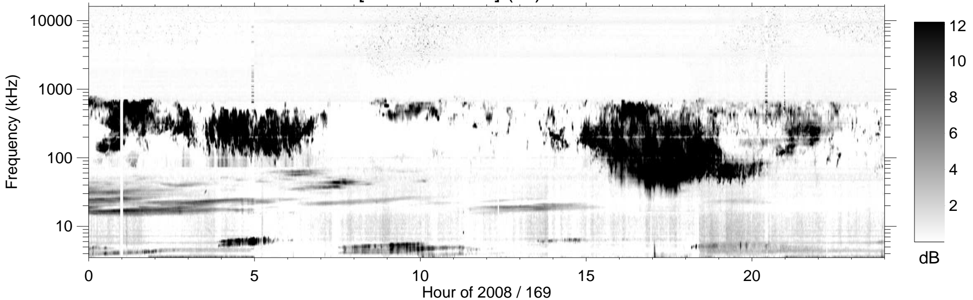
RPWS [ABCH1H2/Ex] (-B) 2008/06/17
