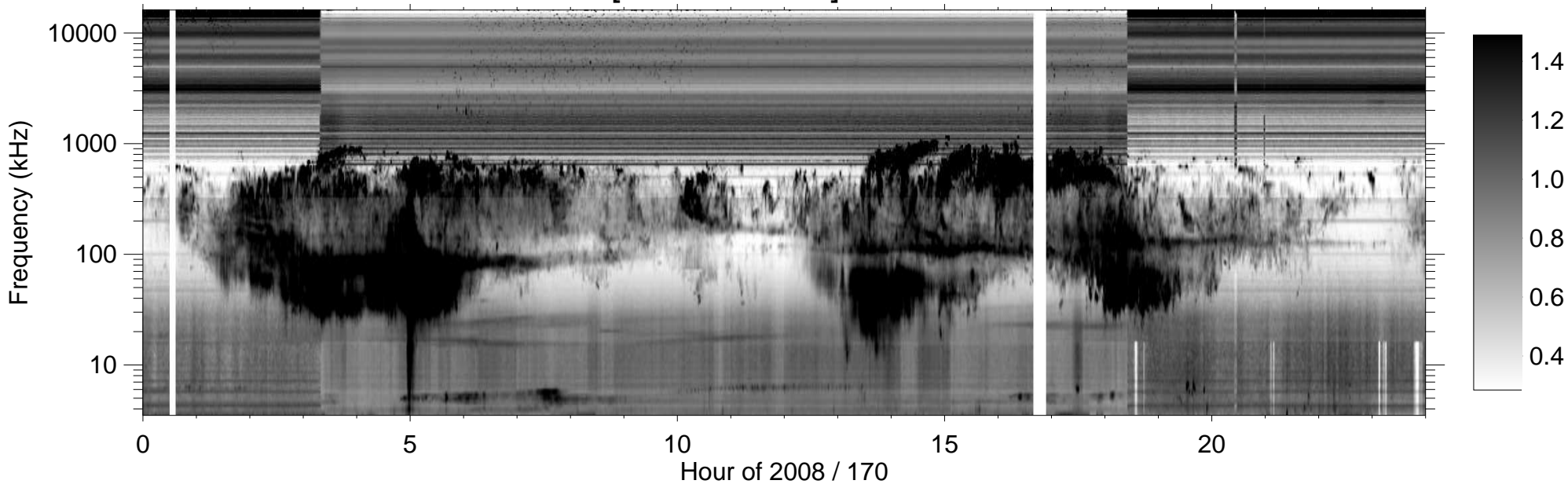
RPWS [ABCH1H2/Ex] (-B) 2008/06/18
