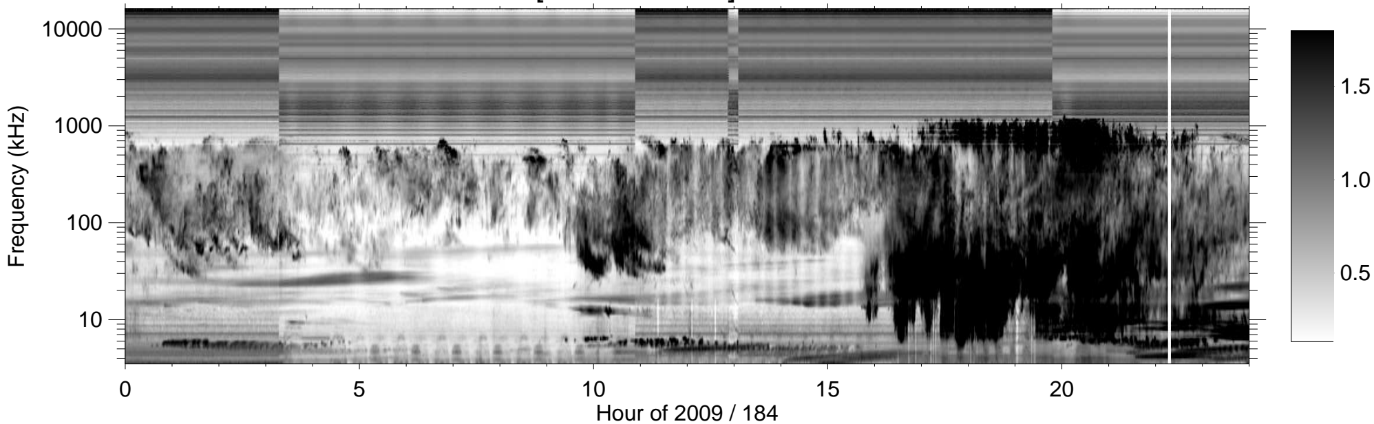
RPWS [ABCH1H2/Ex] (-B) 2009/07/03
