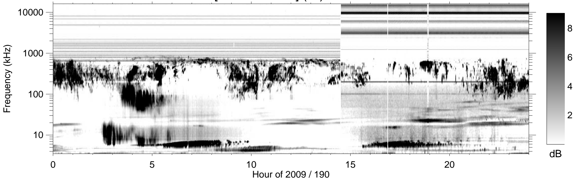
RPWS [ABCH1H2/Ex] (-B) 2009/07/09
