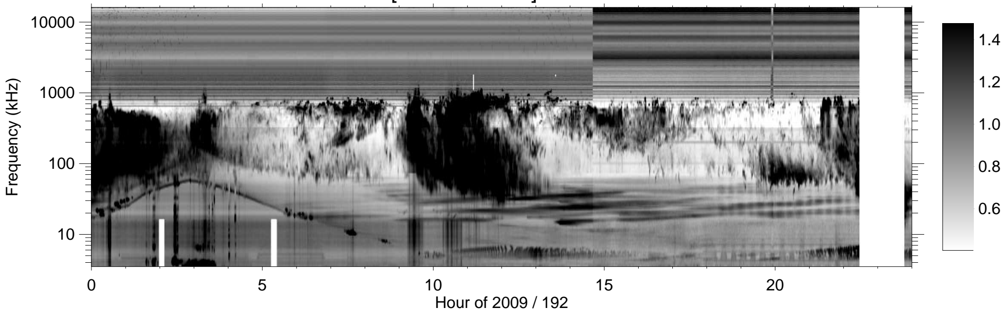
RPWS [ABCH1H2/Ex] (-B) 2009/07/11
