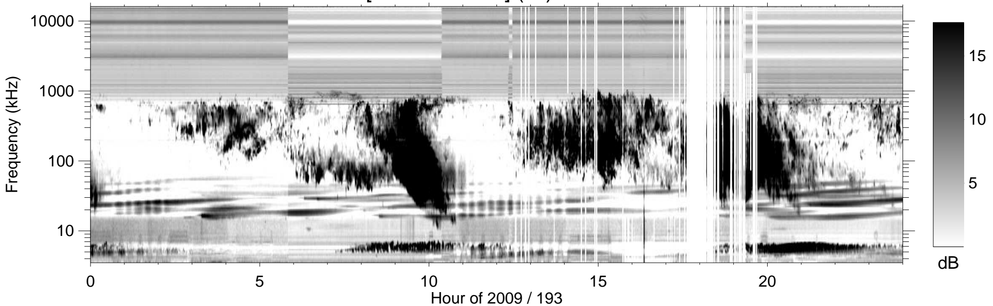
RPWS [ABCH1H2/Ex] (-B) 2009/07/12
