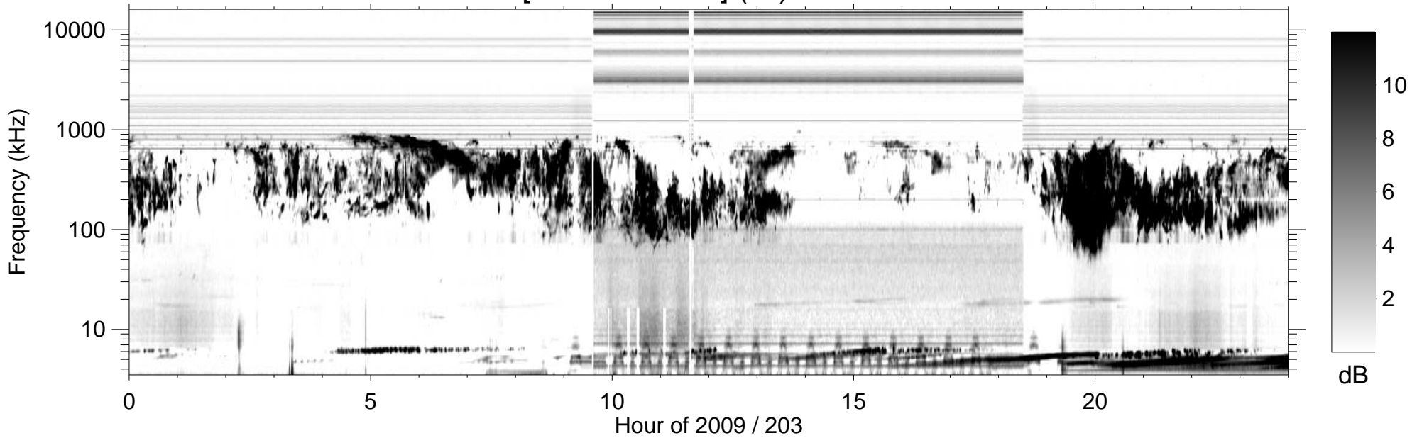
RPWS [ABCH1H2/Ex] (-B) 2009/07/22
