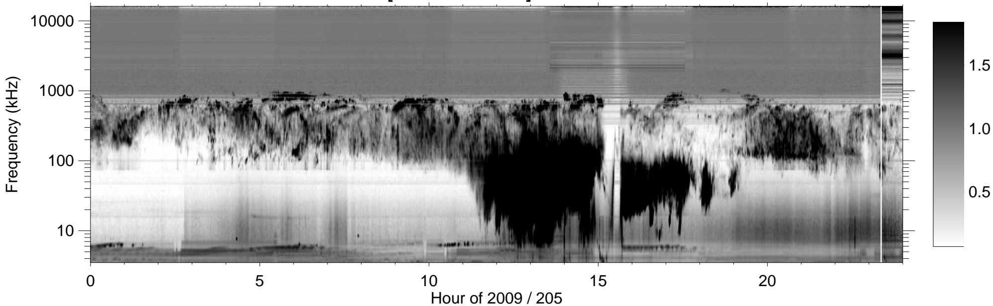
RPWS [ABCH1H2/Ex] (-B) 2009/07/24
