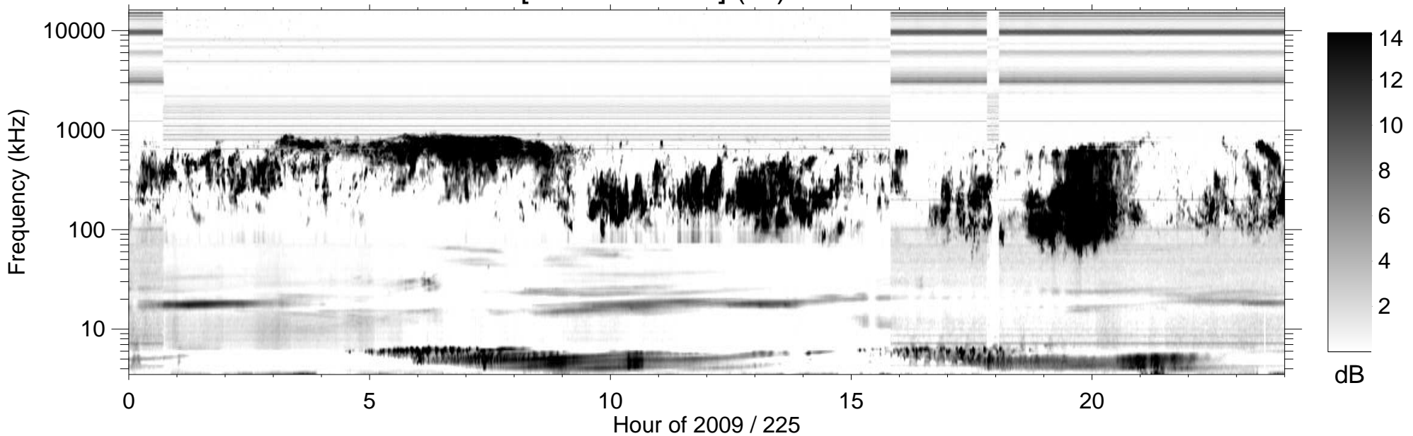
RPWS [ABCH1H2/Ex] (-B) 2009/08/13
