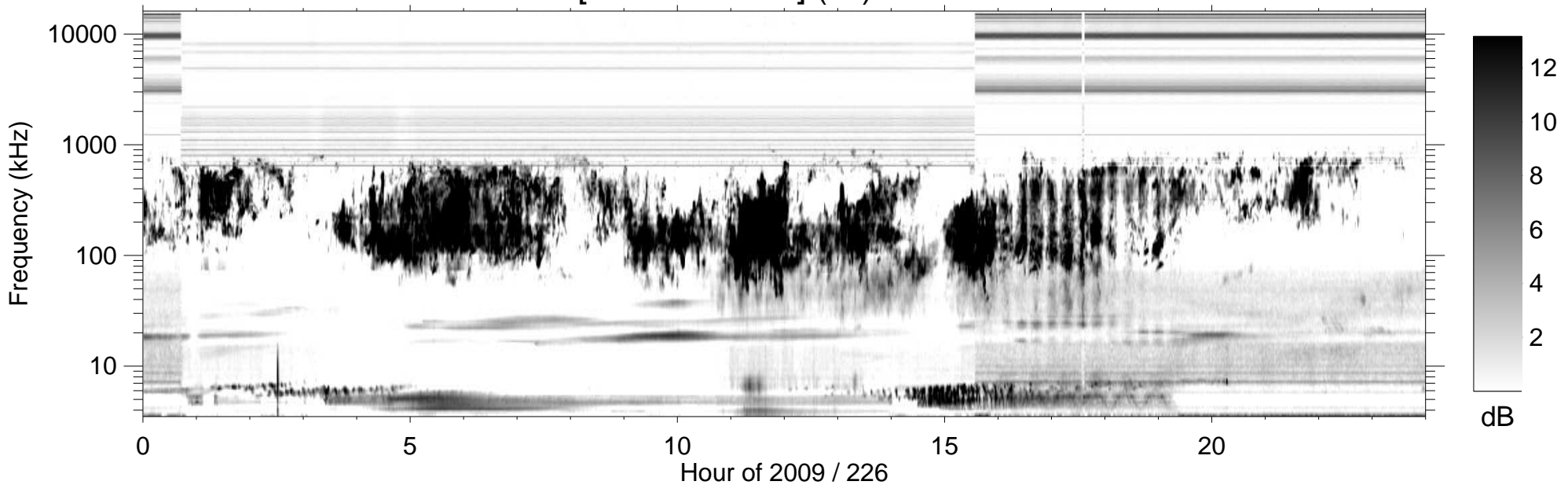
RPWS [ABCH1H2/Ex] (-B) 2009/08/14
