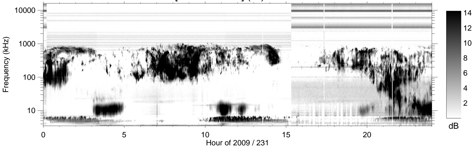
RPWS [ABCH1H2/Ex] (-B) 2009/08/19
