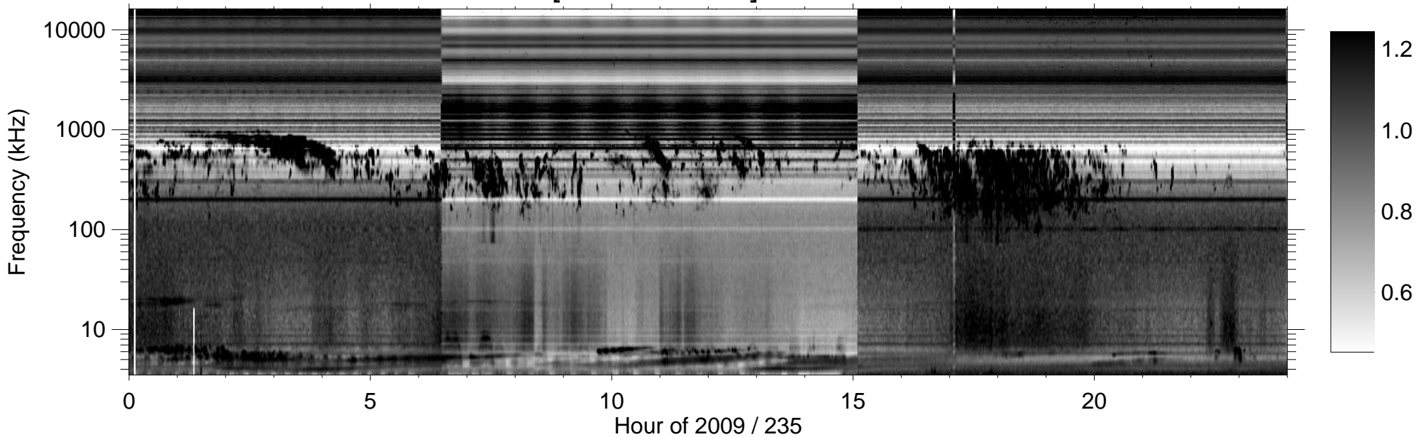
RPWS [ABCH1H2/Ex] (-B) 2009/08/23
