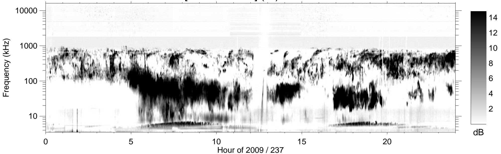
RPWS [ABCH1H2/Ex] (-B) 2009/08/25
