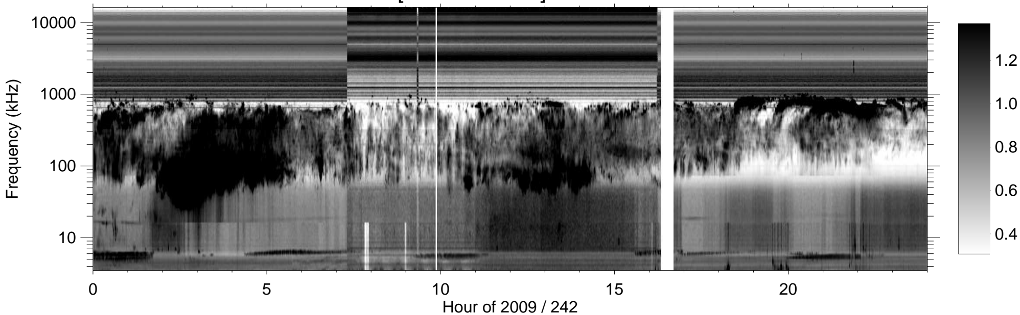
RPWS [ABCH1H2/Ex] (-B) 2009/08/30
