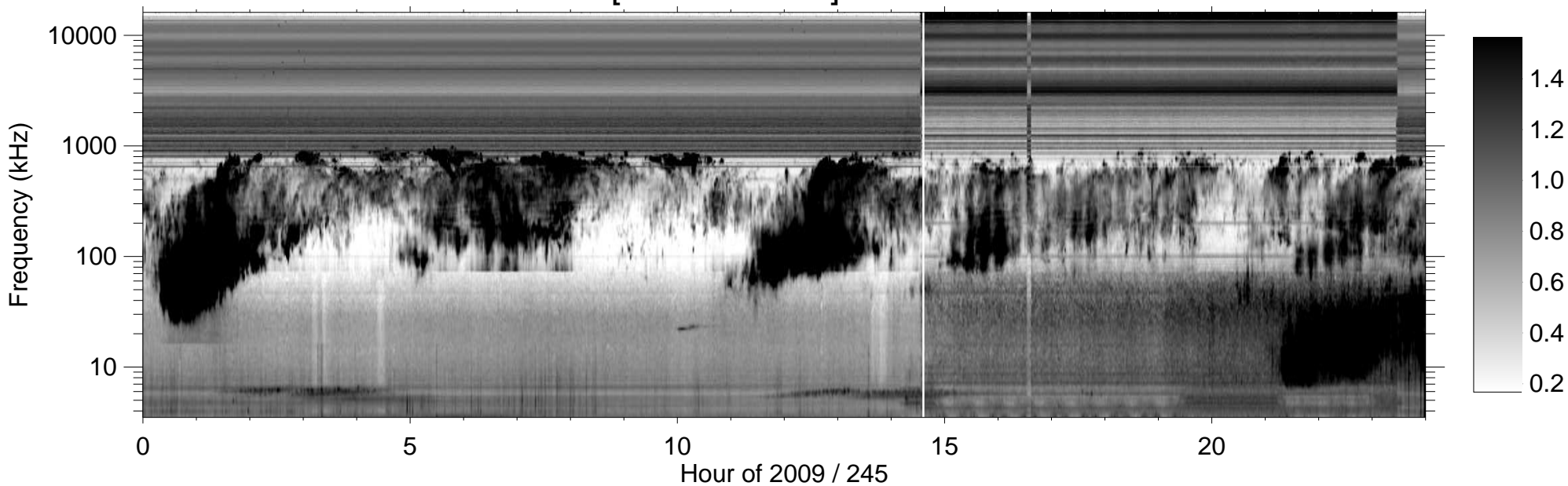
RPWS [ABCH1H2/Ex] (-B) 2009/09/02
