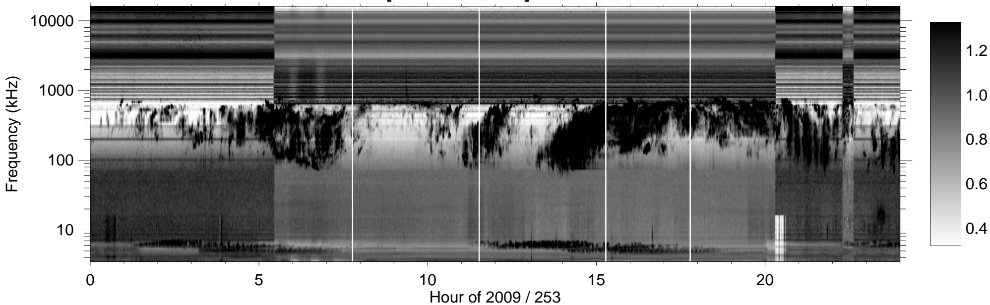
RPWS [ABCH1H2/Ex] (-B) 2009/09/10
