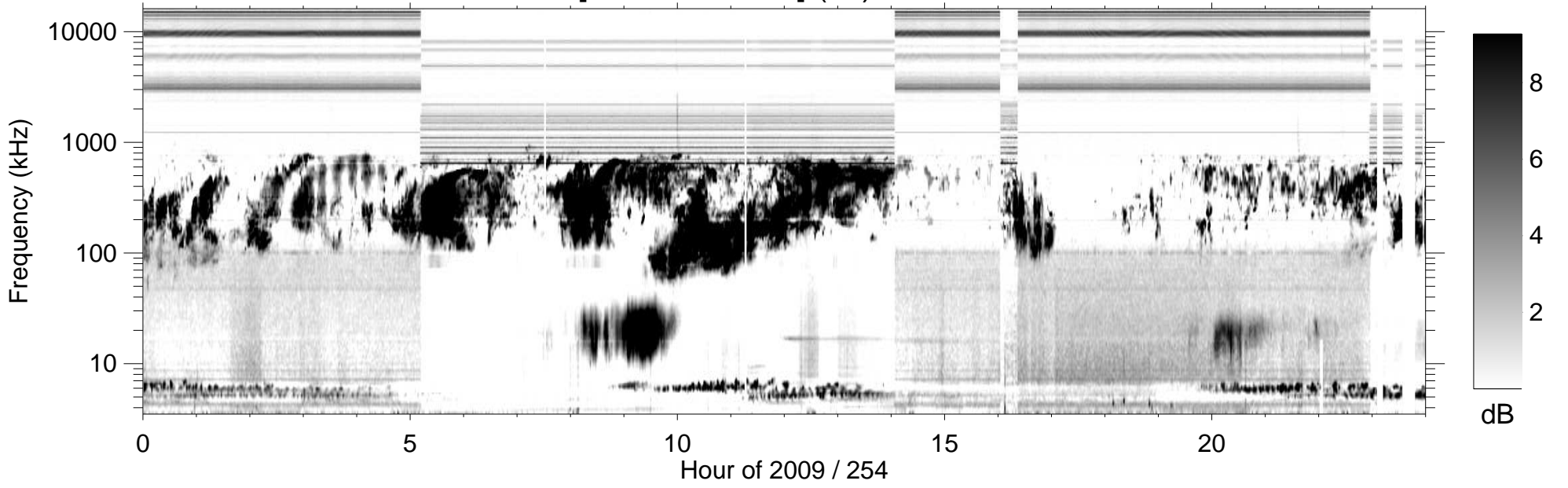
RPWS [ABCH1H2/Ex] (-B) 2009/09/11
