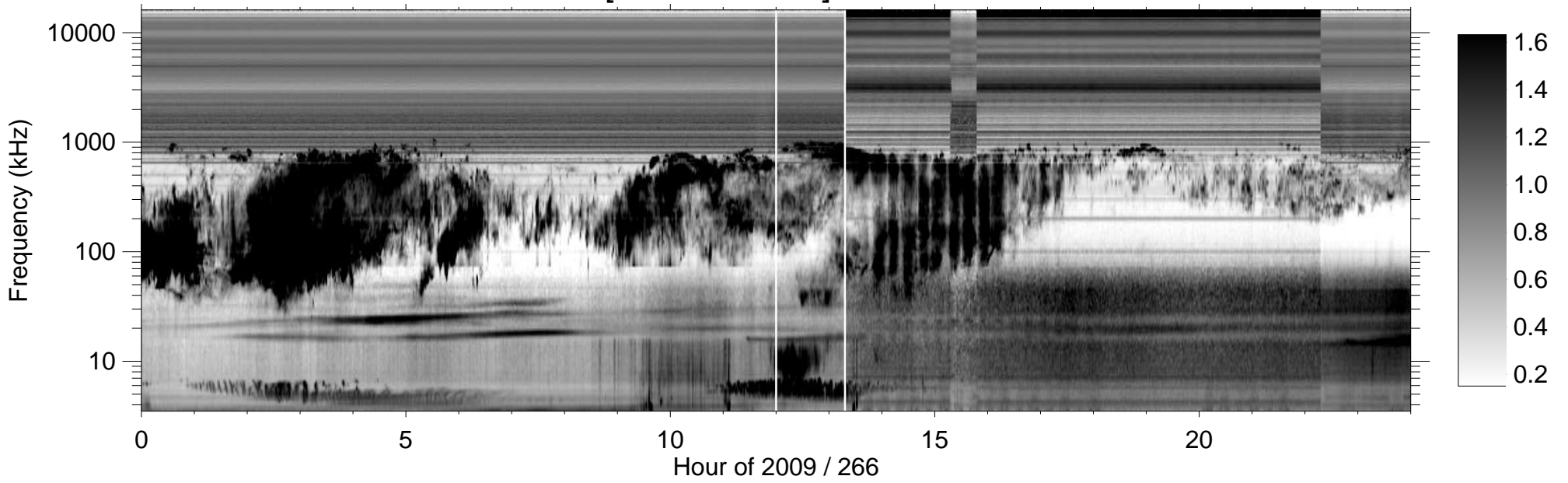
RPWS [ABCH1H2/Ex] (-B) 2009/09/23
