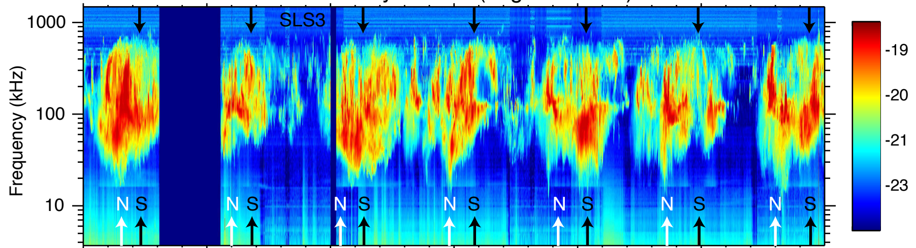
Circular polarization
