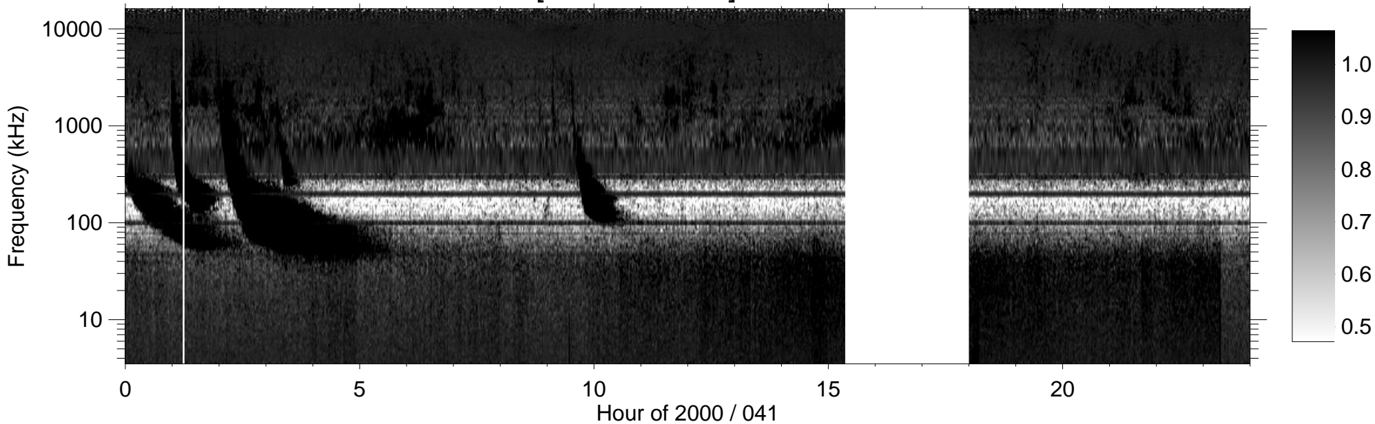
RPWS [ABCH1H2/Ex] (-B) 2000/02/10
