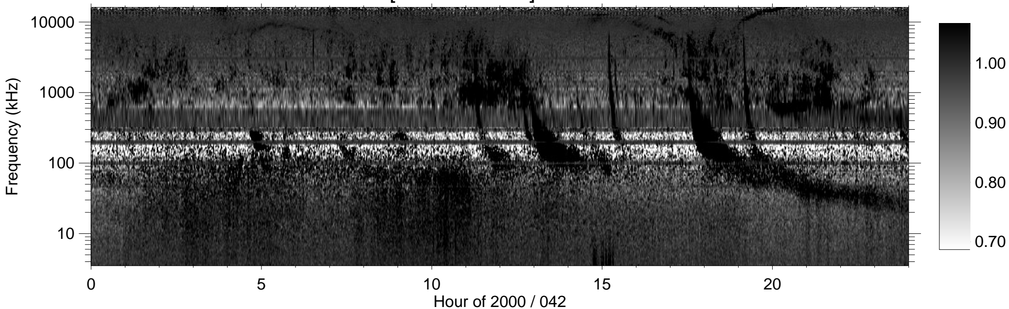
RPWS [ABCH1H2/Ex] (-B) 2000/02/11
