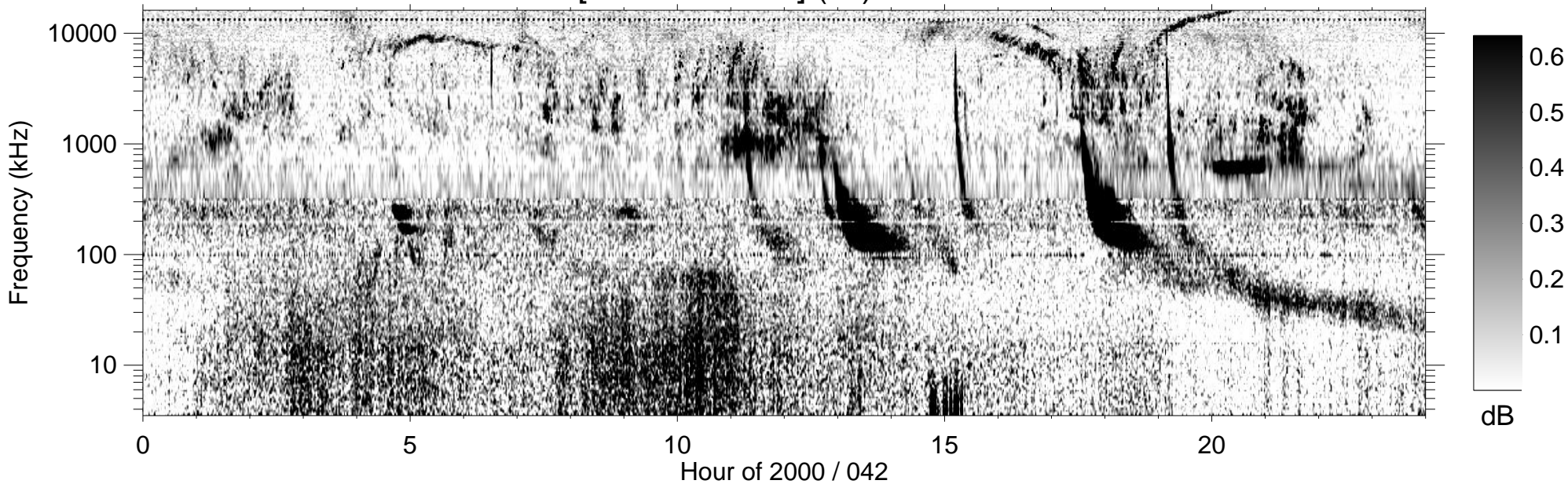
RPWS [ABCH1H2/Ex] (-B) 2000/02/11
