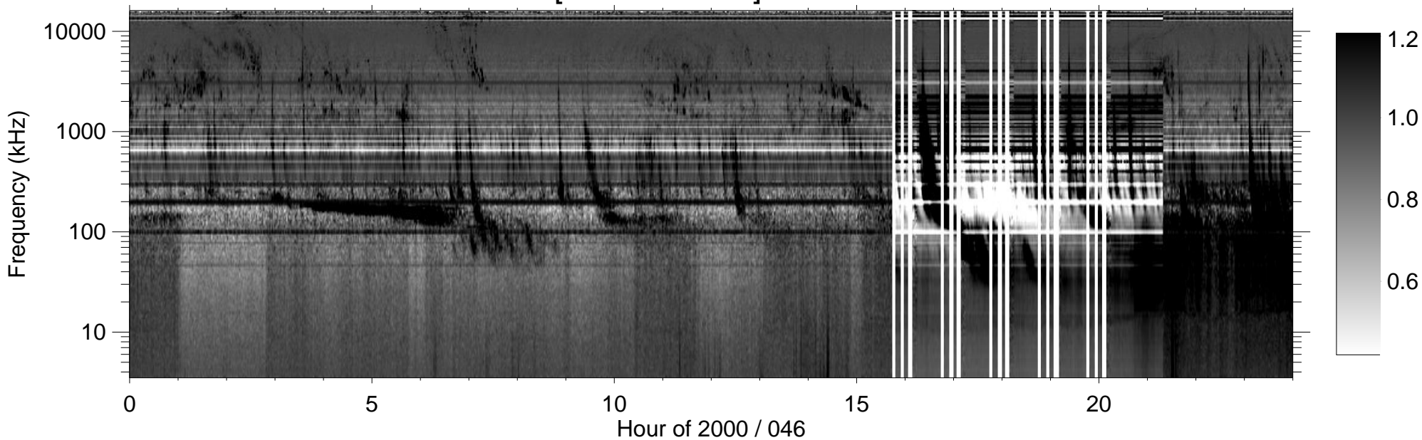
RPWS [ABCH1H2/Ex] (-B) 2000/02/15
