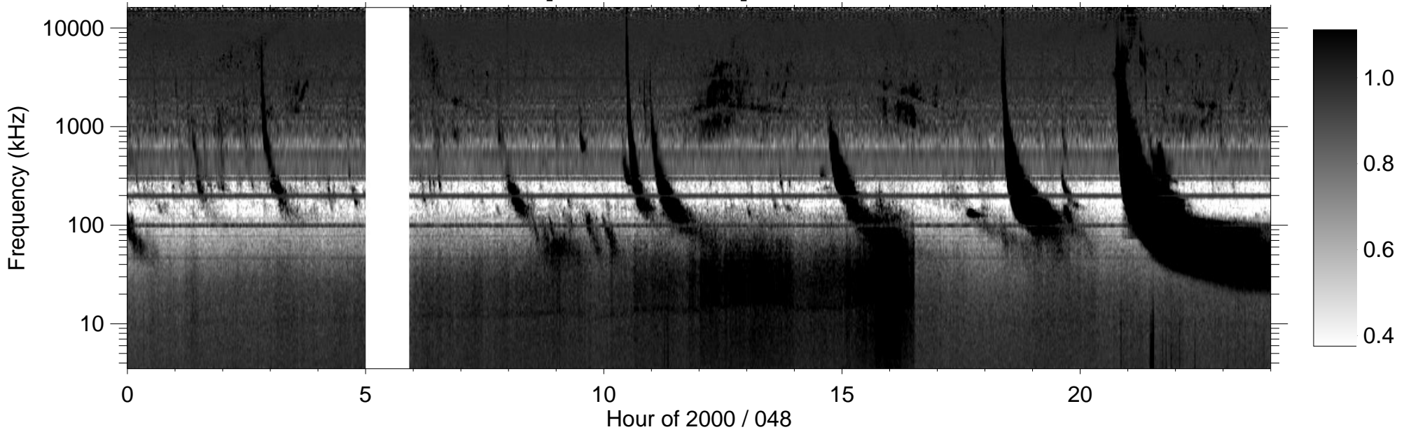
RPWS [ABCH1H2/Ex] (-B) 2000/02/17
