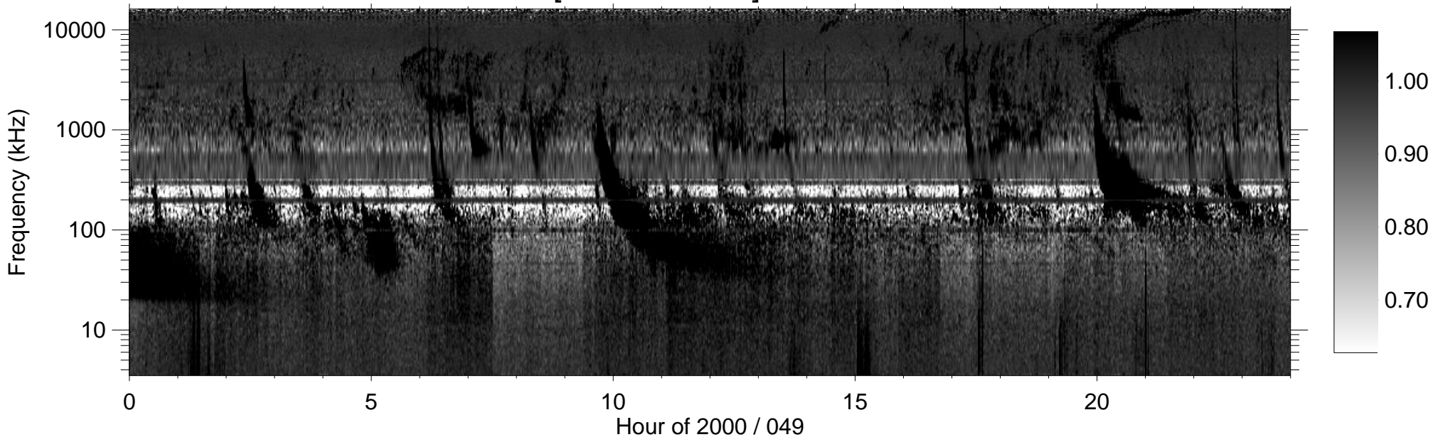
RPWS [ABCH1H2/Ex] (-B) 2000/02/18
