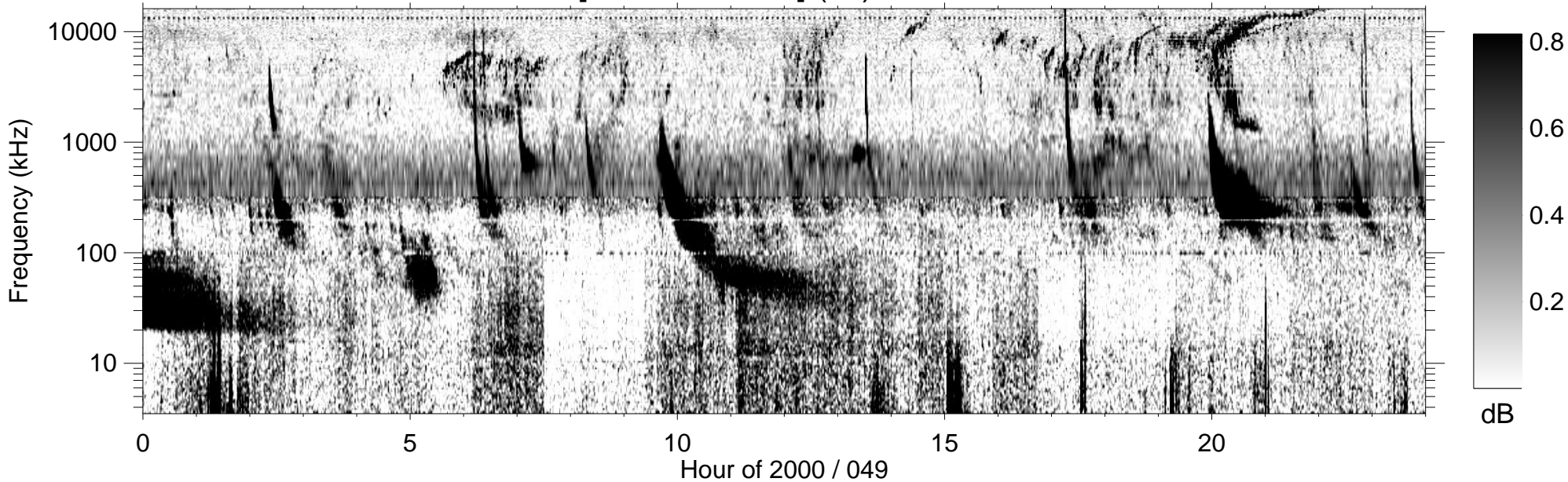
RPWS [ABCH1H2/Ex] (-B) 2000/02/18
