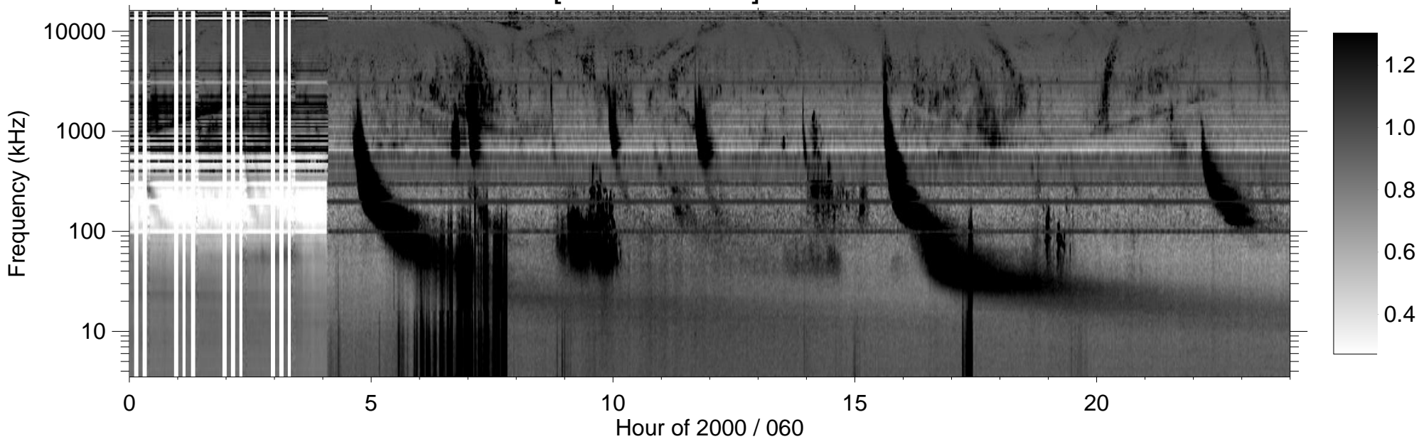
RPWS [ABCH1H2/Ex] (-B) 2000/02/29
