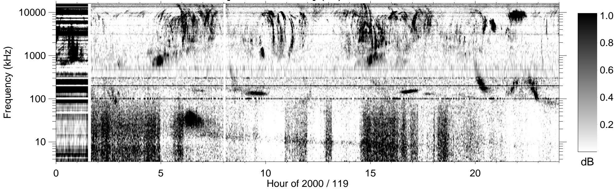
RPWS [ABCH1H2/Ex] (-B) 2000/04/28
