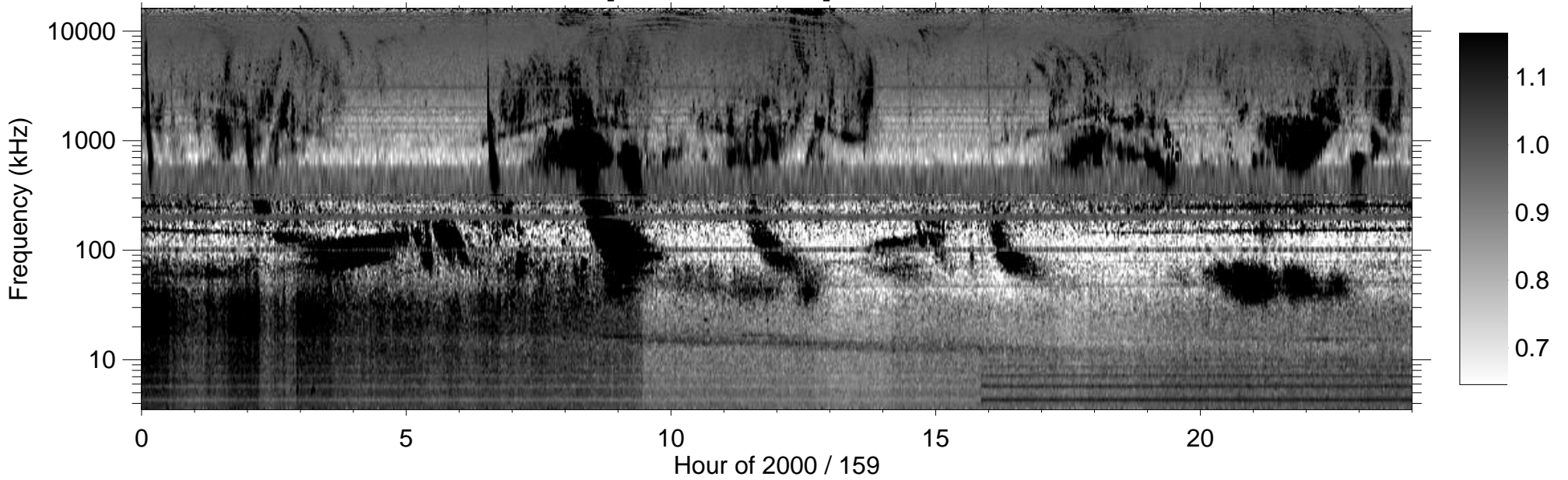
RPWS [ABCH1H2/Ex] (-B) 2000/06/07
