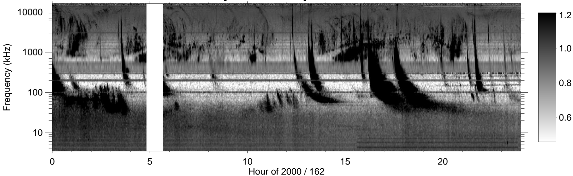
RPWS [ABCH1H2/Ex] (-B) 2000/06/10
