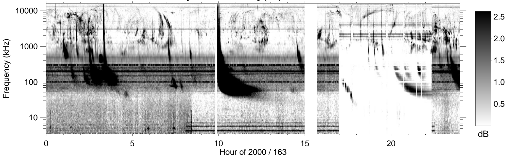
RPWS [ABCH1H2/Ex] (-B) 2000/06/11
