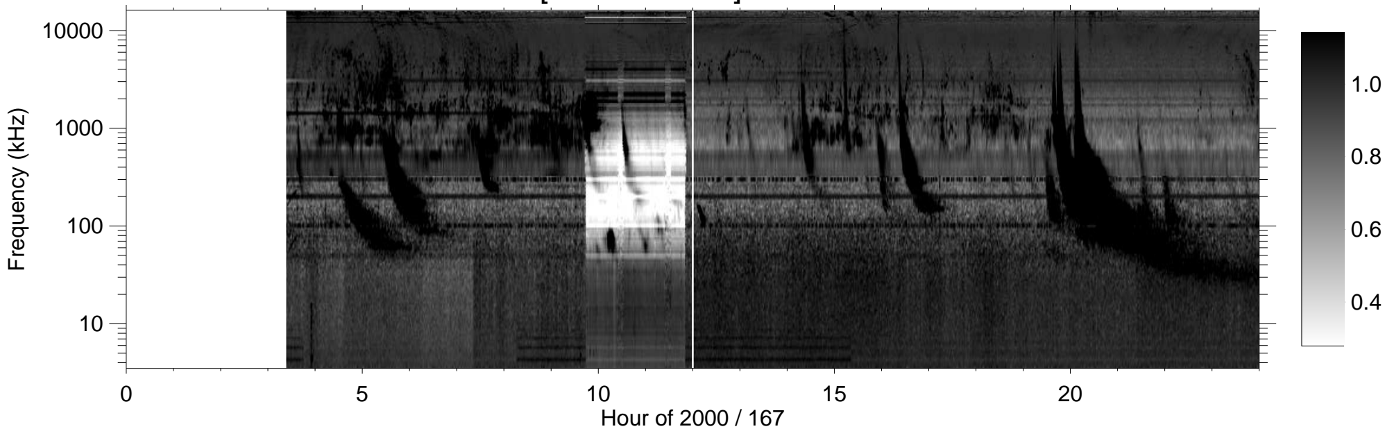
RPWS [ABCH1H2/Ex] (-B) 2000/06/15
