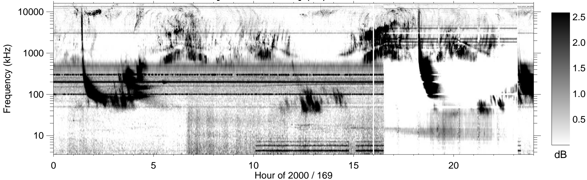
RPWS [ABCH1H2/Ex] (-B) 2000/06/17
