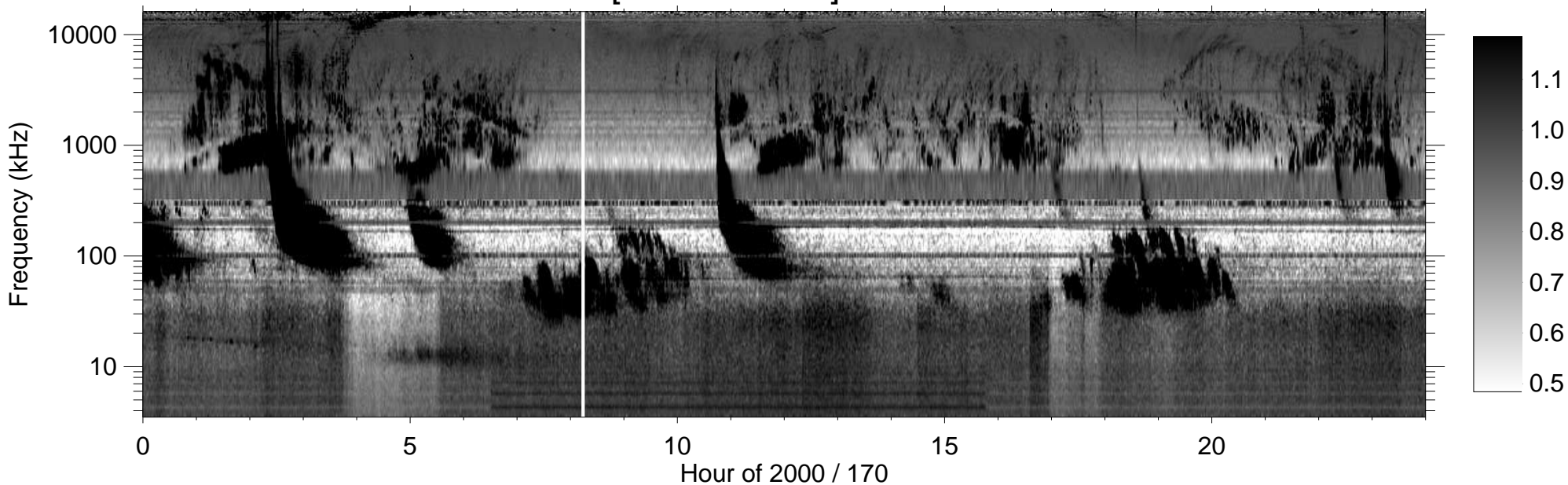
RPWS [ABCH1H2/Ex] (-B) 2000/06/18
