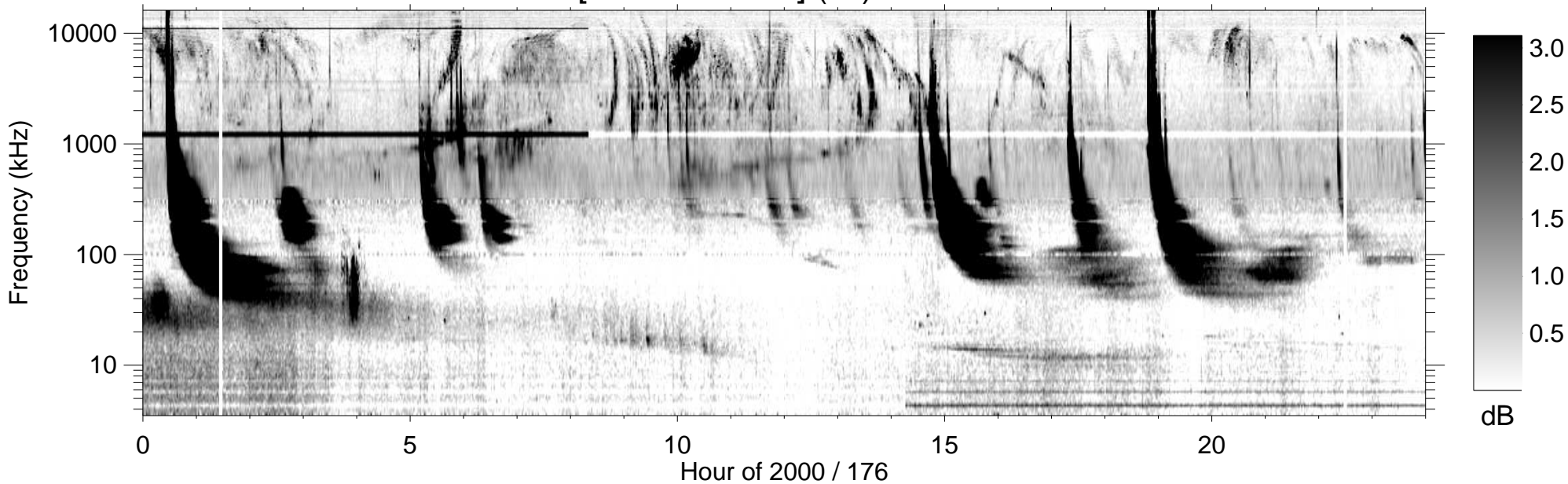
RPWS [ABCH1H2/Ex] (-B) 2000/06/24
