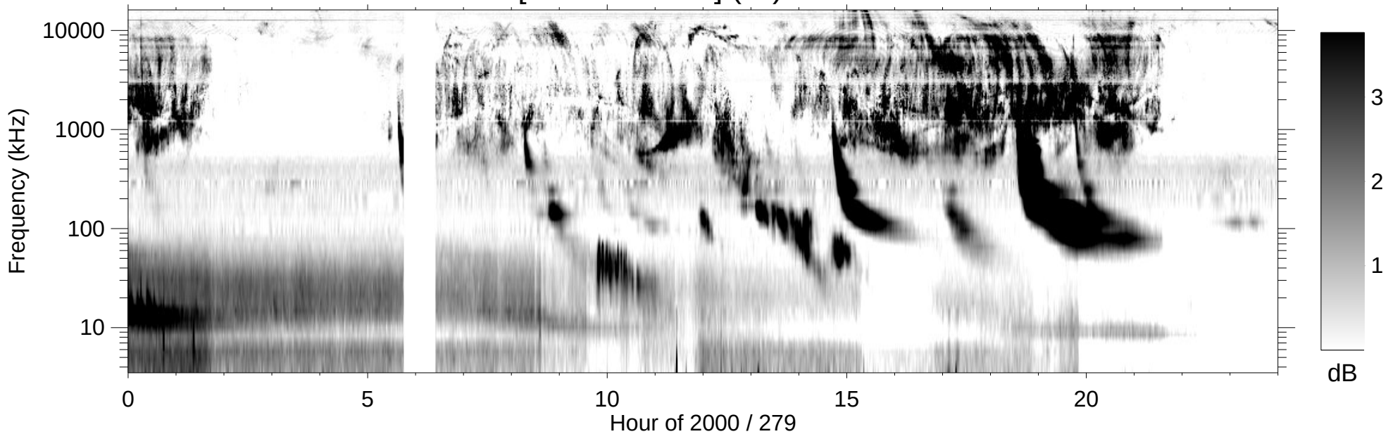
RPWS [ABCH1H2/Ex] (-B) 2000/10/05
