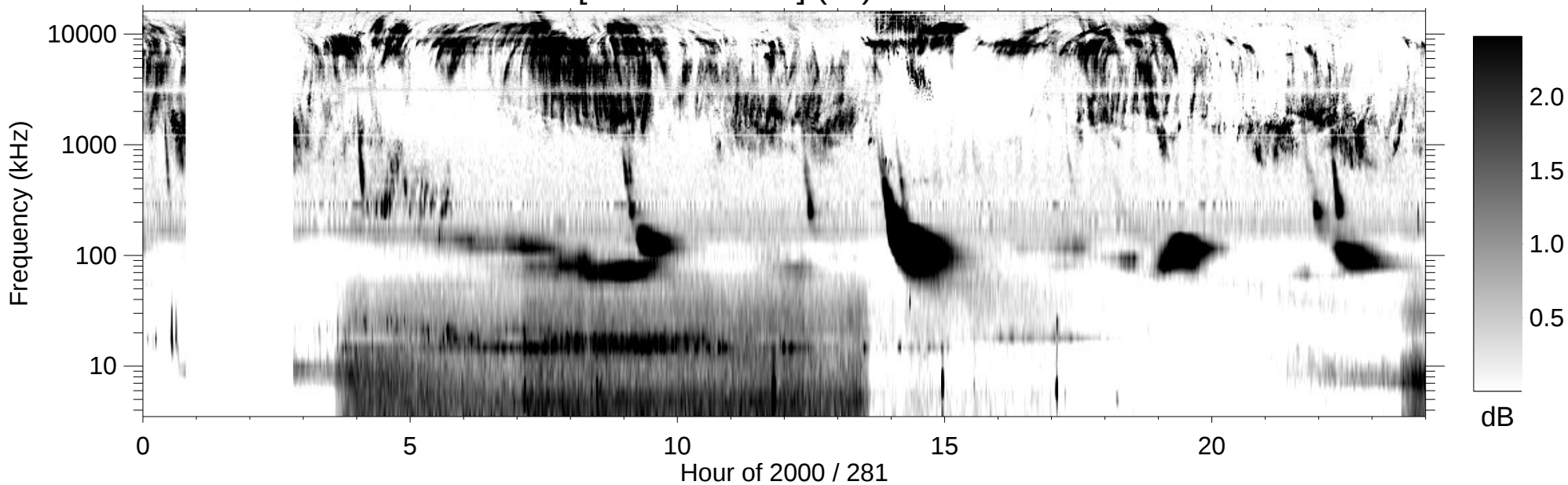
RPWS [ABCH1H2/Ex] (-B) 2000/10/07
