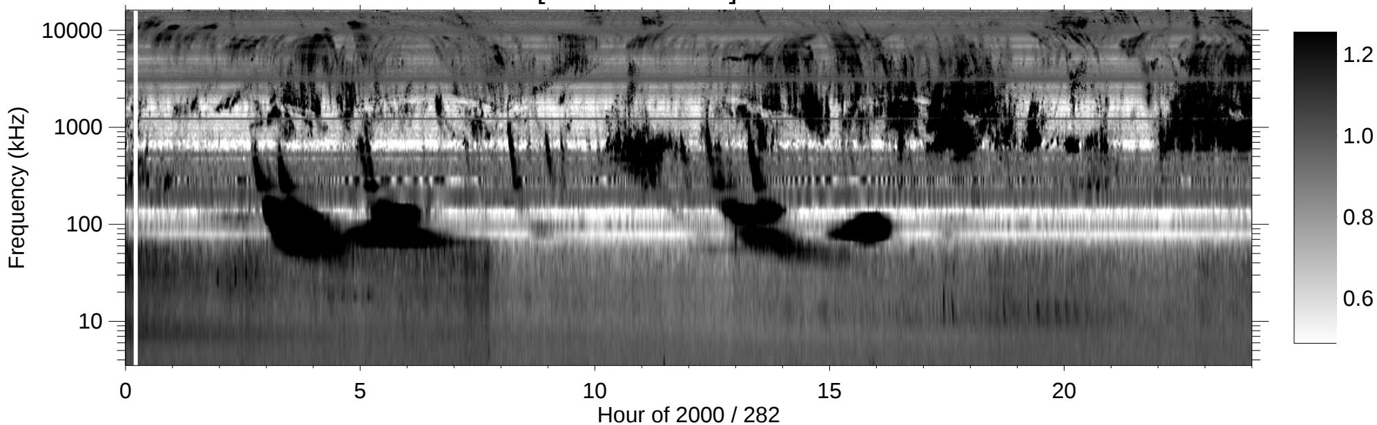
RPWS [ABCH1H2/Ex] (-B) 2000/10/08
