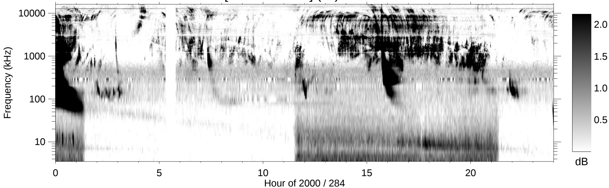
RPWS [ABCH1H2/Ex] (-B) 2000/10/10
